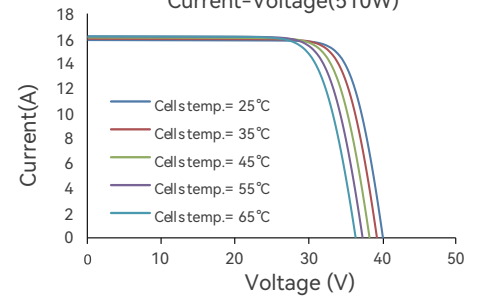
Current-Voltage(510W)
