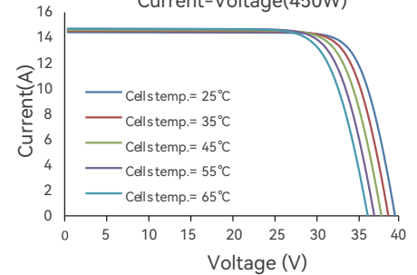
Current-Voltage(450W)
