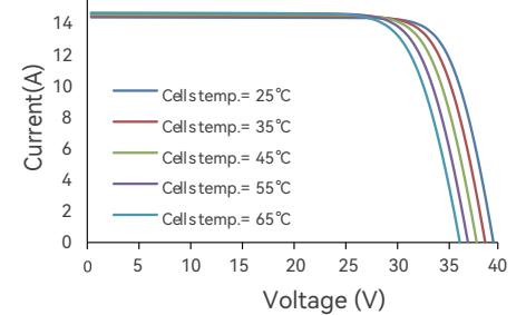
Current-Voltage(450W)
