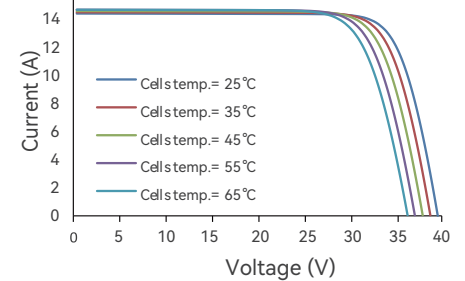
Current-Voltage(450W)
