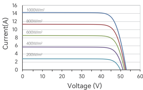
Current-Voltage(600W)
