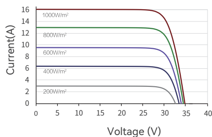
Current-Voltage(455W)
