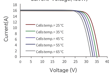
Current-Voltage(455W)
