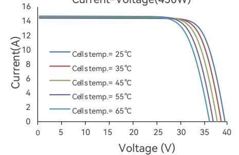
Current-Voltage(450W)
