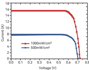
IVcurve
