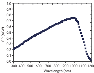
QEcurve
