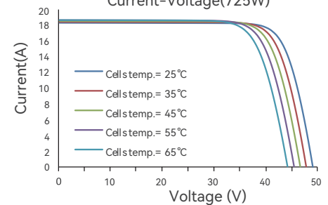
Current-Voltage(725W)
