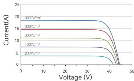
Current-Voltage(725W)
