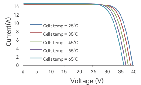
Current-Voltage(450W)
